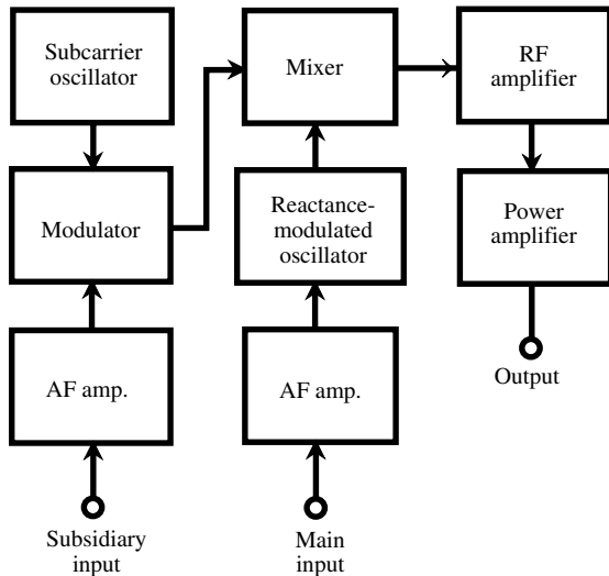
multiplexing, 1.
