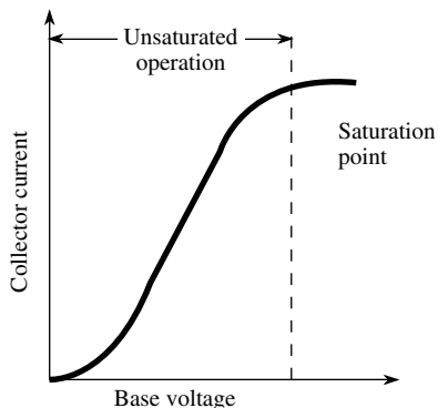
unsaturated operation
