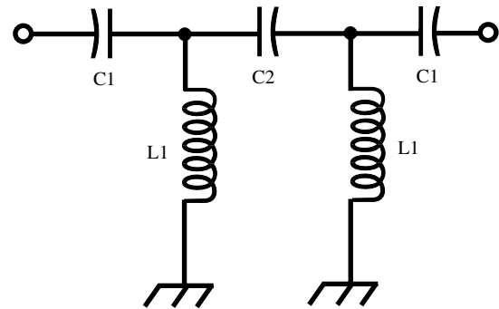
bilateral network
