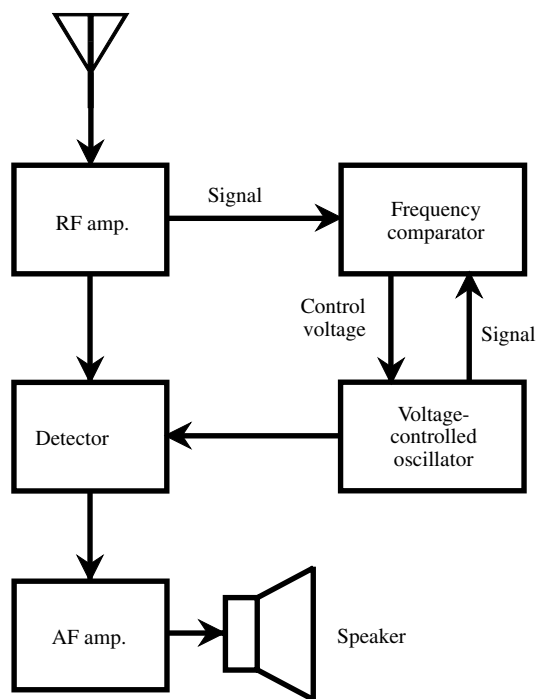
synchrodyne receiver
