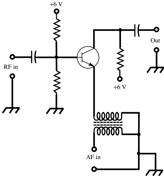
modulated amplifier
