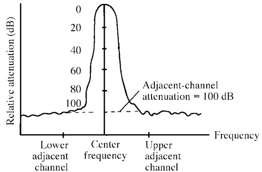
adjacent-channel attenuation
