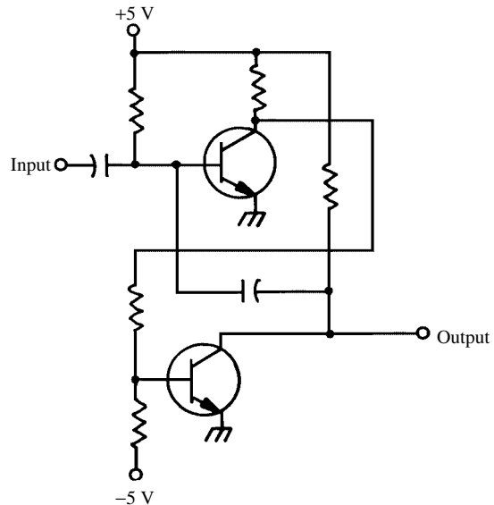
monostable multivibrator
