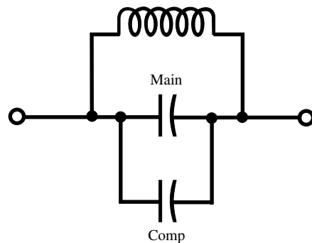
compensating capacitor, 1.
