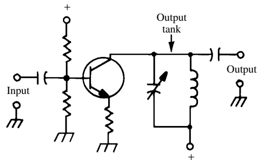
output tank
