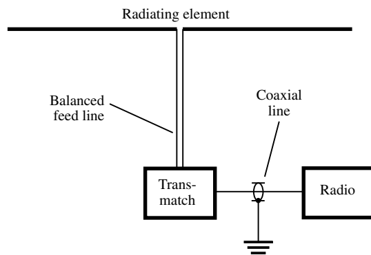
multiband antenna
