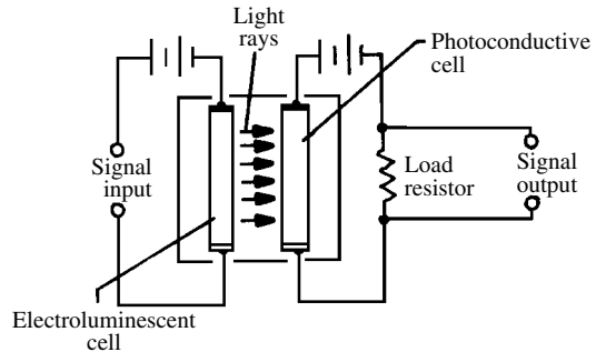
lumistor
