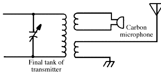
absorption modulation
