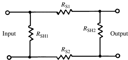
O network
