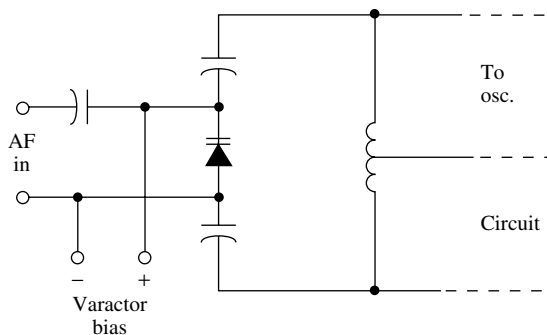
reactance modulator
