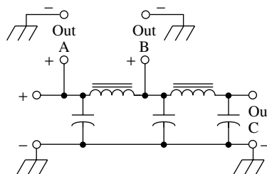
graded filter
