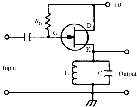
shock-excited oscillator
