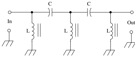
high-pass filter
