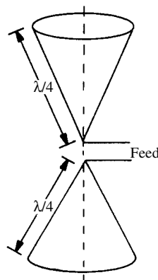
biconical antenna
