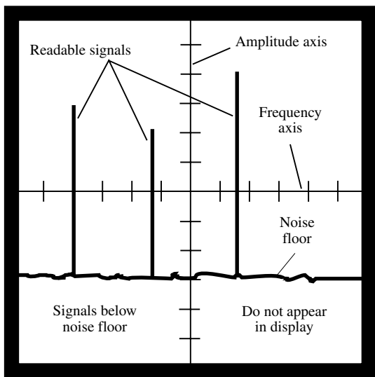
noise floor, 2.
