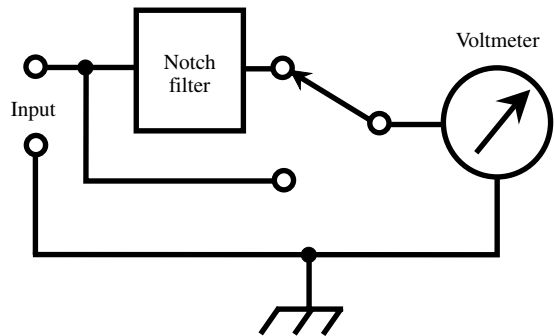
distortion meter
