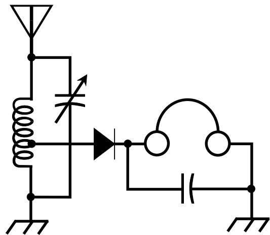
crystal set
