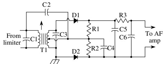
discriminator
