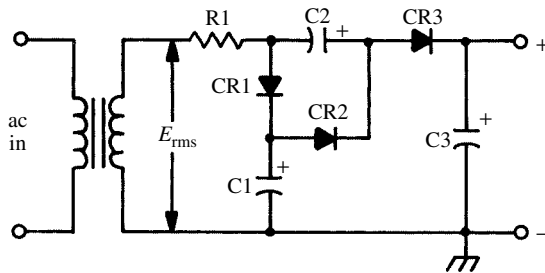
tripler, 1
