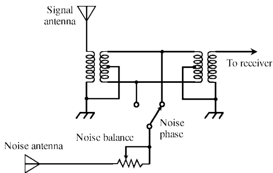
noise-canceling antenna
