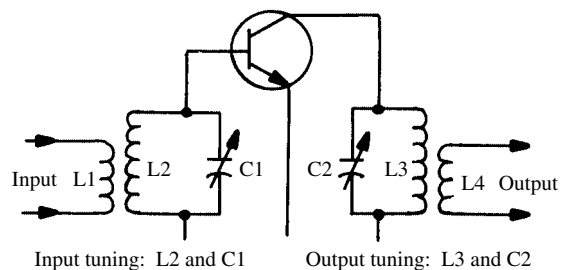
double-tuned circuit
