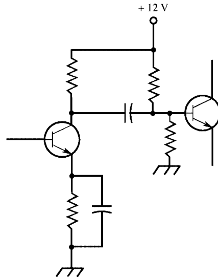
bypass capacitor
