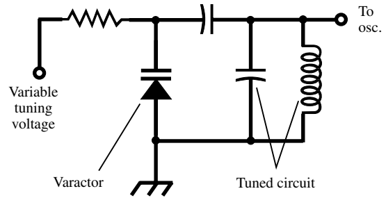
electric tuning
