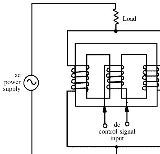
magnetic amplifier
