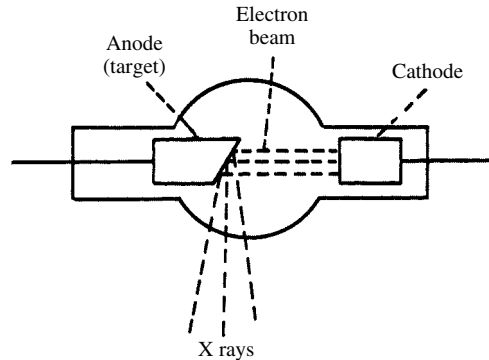
X-ray tube
