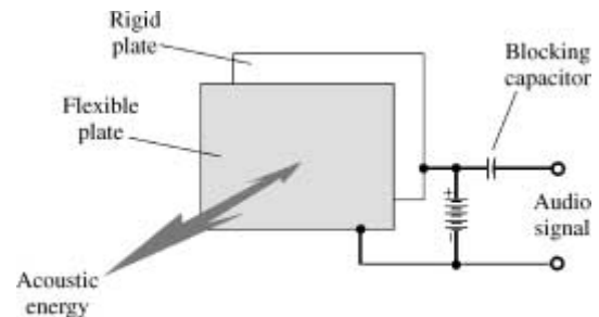
electrostatic speaker
