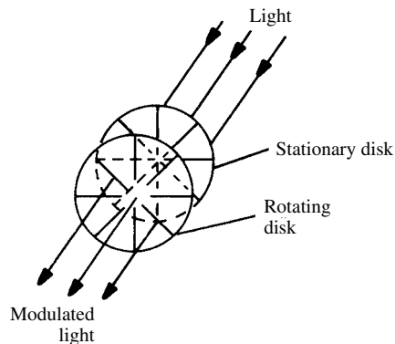
episcotister
