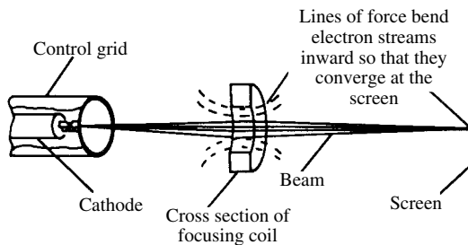
electromagnetic focusing
